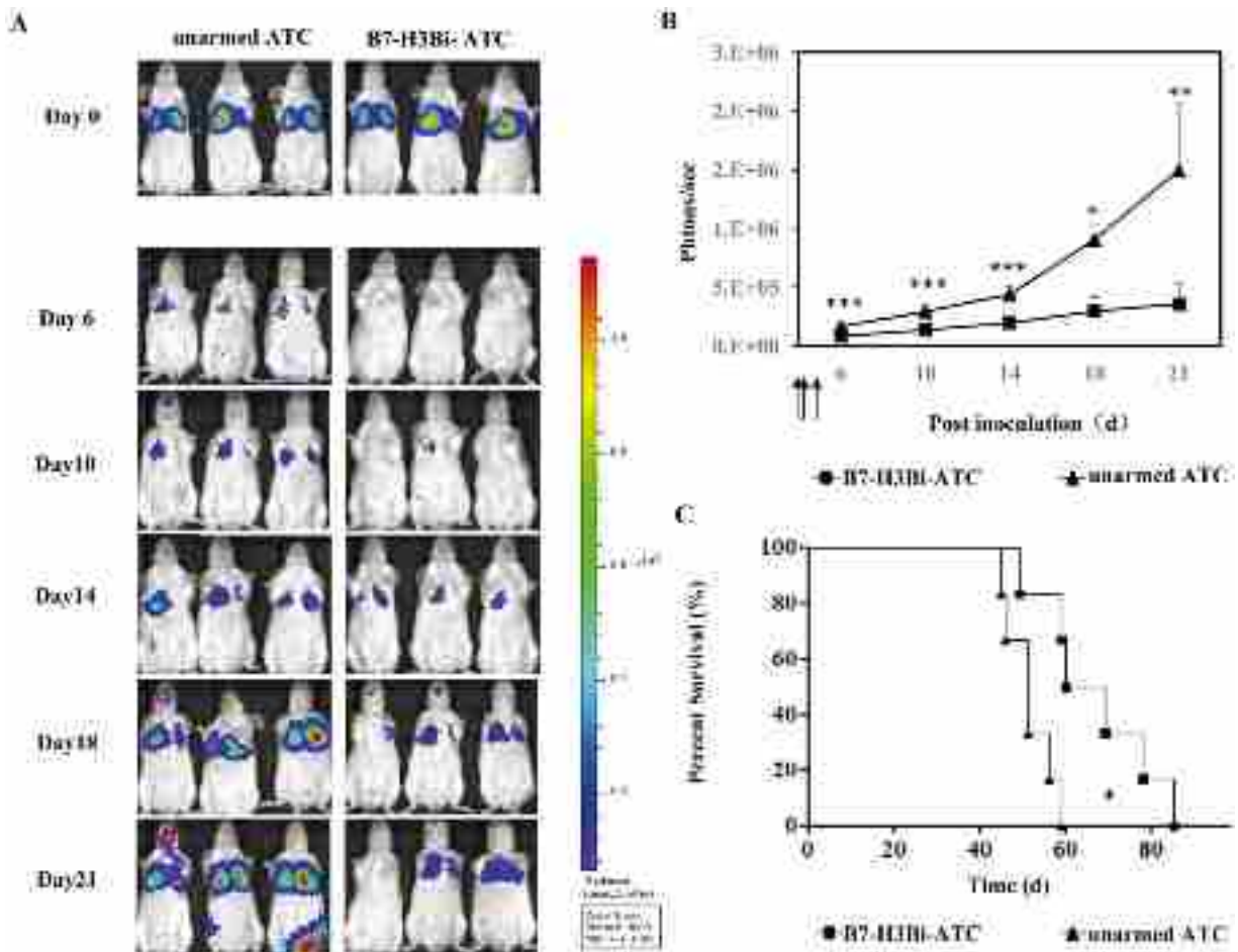
Figure 6: In vivo anti-tumor potency of B7-H3Bi-armed ATC in mouse lung cancer metastasis model. SCID/Beige mice were inoculated intravenously with 2 \times 10^6 A549-luc cells. On day 0, day 1 and day 3, tumor-bearing mice were administrated i.v. with 2 \times 10^7 B7-H3Bi-armed ATC or unarmed ATC respectively (each group contains 5 mice). Tumor growth was monitored using an in vivo imaging system A . Bioluminescence images of 3 representative mice of each group were shown on indicated day. B . Images were analyzed using Living Image software and tumor values represented as total flux measurements in photons/second, mean values of tumor growth curves were shown. C . Survival curves of mice engrafted with A549-luc cells receiving B7-H3Bi-armed ATC or unarmed ATC were shown. * P < 0.05 , ** P < 0.01 , *** P < 0.001 , B7-H3Bi-armed ATC was compared with unarmed ATC under similar conditions.
