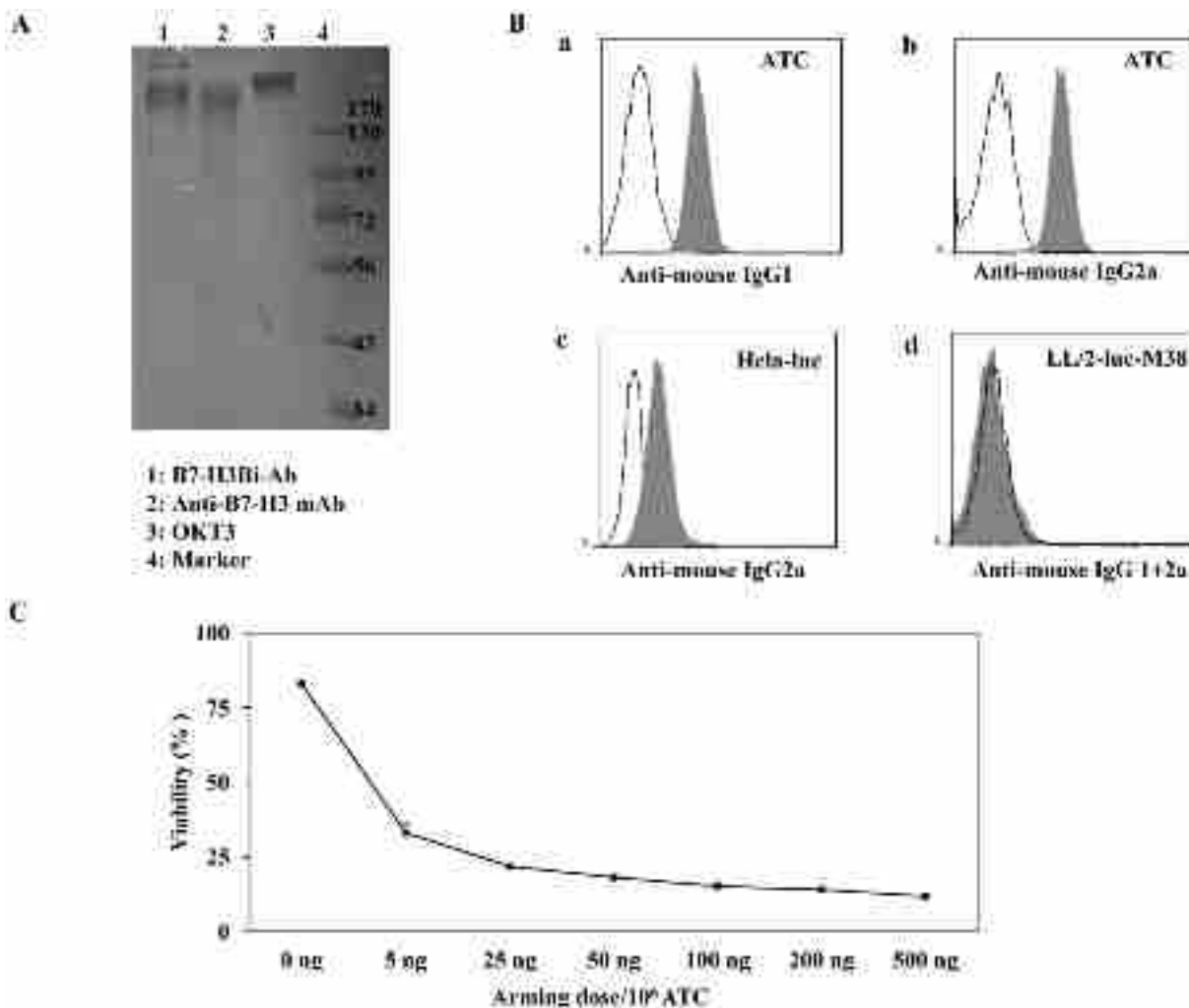
Figure 2: Generation of anti-CD3 × anti-B7-H3 bispecific antibody (B7-H3Bi-Ab). A. The heteroconjugated product of equimolar concentrations of B7-H3Bi-Ab was quantified by Coomassie blue staining of SDS-gel. B. Flow cytometry based binding assay for B7-H3Bi-Ab was tested. ATC was stained by B7-H3Bi-Ab (shaded histogram), or a combination of OKT3 with anti-B7-H3 (the black line), then FITC-anti-mouse-IgG1 was added to detect the B7-H3 moiety of B7-H3Bi-Ab (a), or an FITC-anti-mouse IgG2a to detect the anti-CD3 moiety of the B7-H3Bi-Ab (b). (c) HeLa-luc cells were incubated with B7-H3Bi-Ab (shaded histogram) or a combination of OKT3 and anti-B7-H3 (the black line), then B7-H3Bi-Ab binding was confirmed by FITC-anti-mouse IgG2a to detect the anti-CD3 moiety of the B7-H3Bi-Ab. (d) LL/2-luc-M38 cells were incubated with B7-H3Bi-Ab (shaded histogram) or a combination of OKT3 and anti-B7-H3 (the black line), then B7-H3Bi-Ab binding was analyzed by combined FITC-anti-mouse IgG2a with an anti-mouse-IgG1-FITC. C. Titer of B7-H3Bi-Ab armed ATC was measured. ATC was armed with B7-H3Bi-Ab ranging from 5 to 500 ng/10 6 cells at E/T ratio of 10:1, and cytotoxic effects of B7-H3Bi-armed ATC on HeLa-luc cells were tested in vitro. After 18 hour incubation with B7-H3Bi-armed ATC, the percentage of viability was calculated at each concentration.
